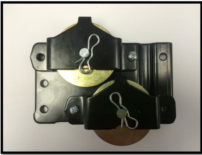
22302 CORNER PULLEY KIT, RH
